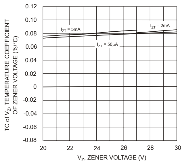
Fig. 17 Typical Temperature Coefficient of Zener Voltage, DDZ20C-DDZ30D
