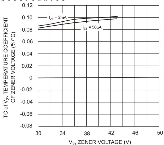
Fig. 18 Typical Temperature Coefficient of Zener Voltage, DDZ30D-DDZ43
