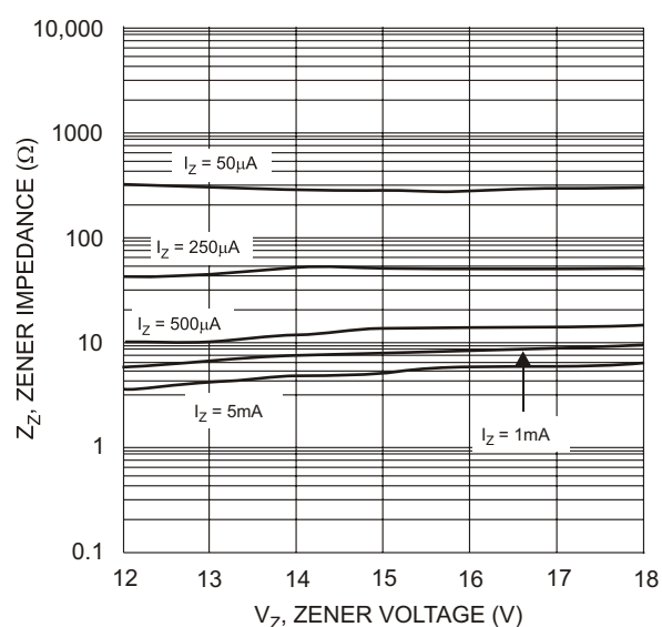
Fig. 11 Typical Zener Impedance Characteristics, DDZ12C - DDZ18C
