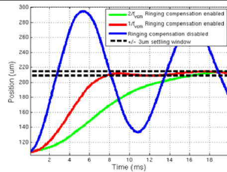
Figure 17. Lens Positions With and Without Ringing Compensation With 100- \mu\text{m} Step on the Lens Position, Zoomed In
