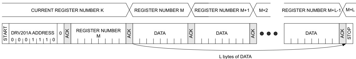
Figure 10. Sequential Write
