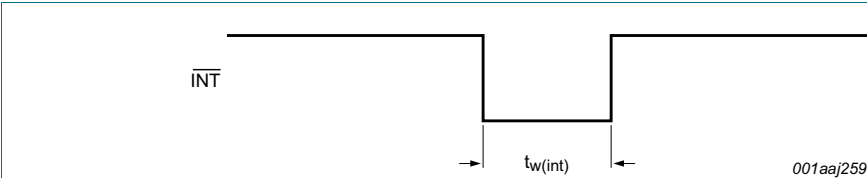
Fig 27. \overline{INT} timing
