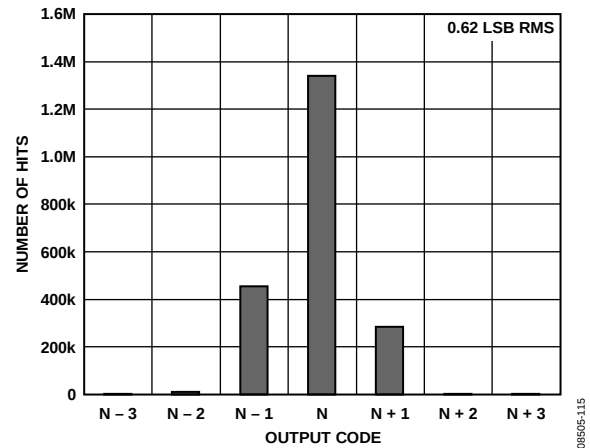
Figure 15. AD9255-80 Grounded Input Histogram
