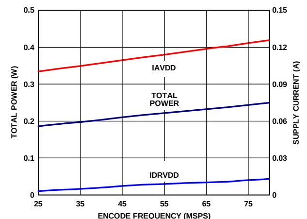
Figure 83. AD9255-80 Power and Current vs. Sample Rate
