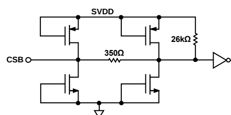
Figure 60. Equivalent CSB Input Circuit
