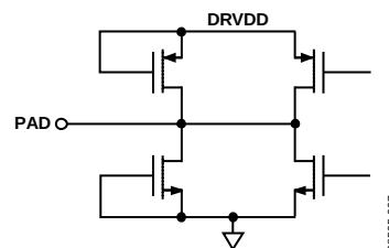
Figure 57. Digital Output
