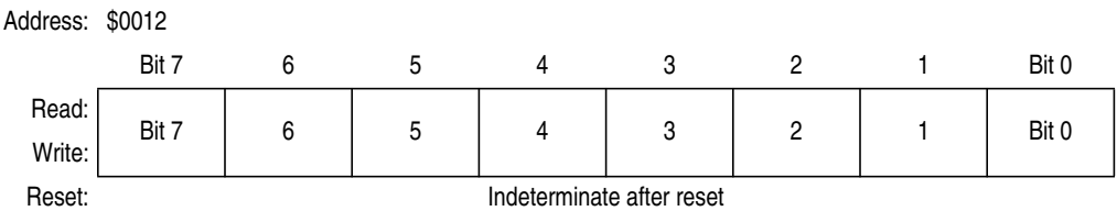
Figure 8-13. TIM Channel 0 Register Low (TCH0L)
