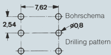
Lage der Anschlüsse Positions of Terminals
