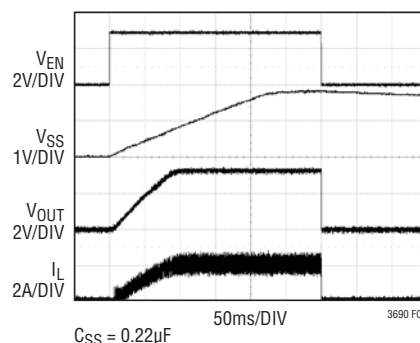
Figure 7. Soft-Start Ramp
