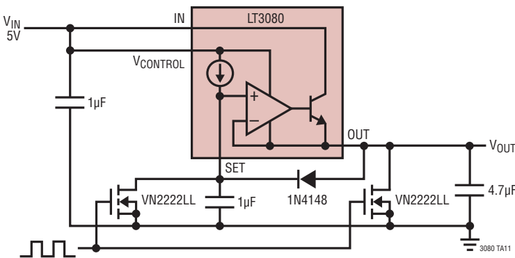
Ramp Generator
