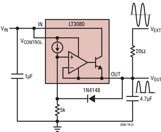
Ground Clamp
