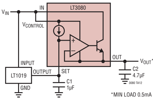
Reference Buffer
