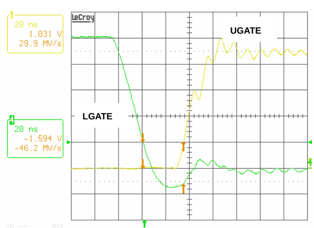
FIGURE 21. GATE DRIVER WAVEFORMS AT V_{IN} = 8V , I_{LOAD} = 40A , 2-PHASE MODE. 2 X IRF7821 AS UPPER DEVICE AND 2 X IRF7832 AS LOWER DEVICE
