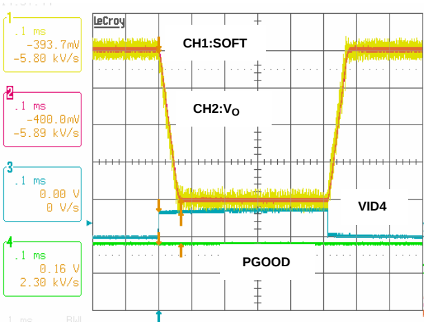
FIGURE 20. VID TRANSITION RESPONSE AT 2-PHASE CCM MODE, V_{IN} = 12.6V AND V_{ID} = 1.55V \rightarrow 1.15V
