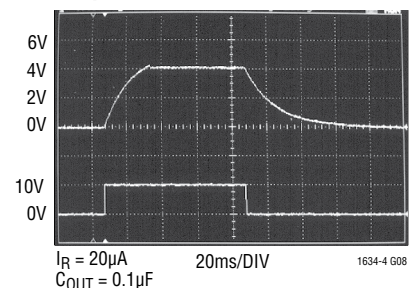
Response Time
