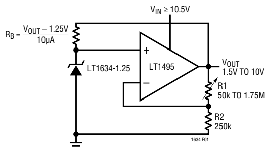
Figure 1. Adjustable Output Voltage Reference
