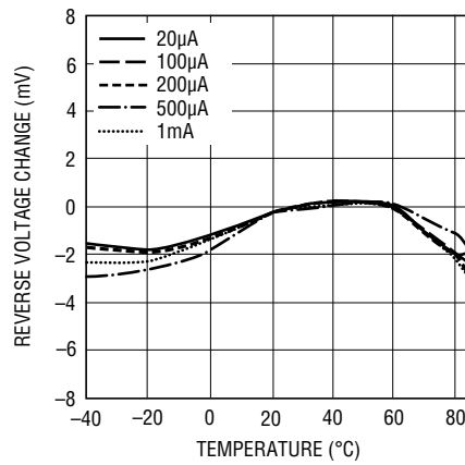
Temperature Drift
