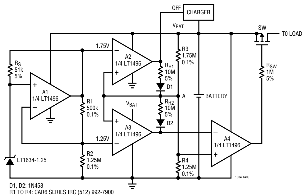
Single Cell Li-Ion Battery Supervisory Circuit (I Q = 20μA)
