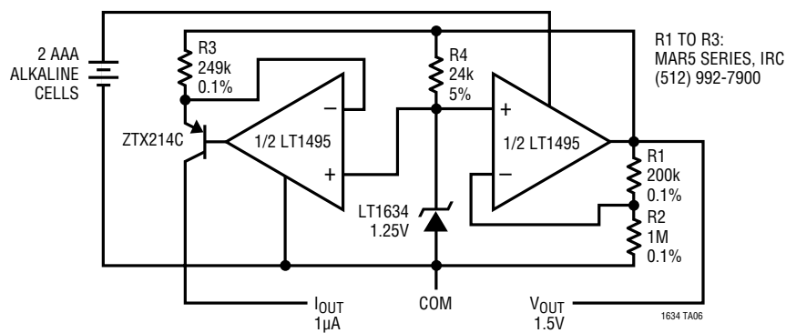
Micropower Voltage and Current Reference
