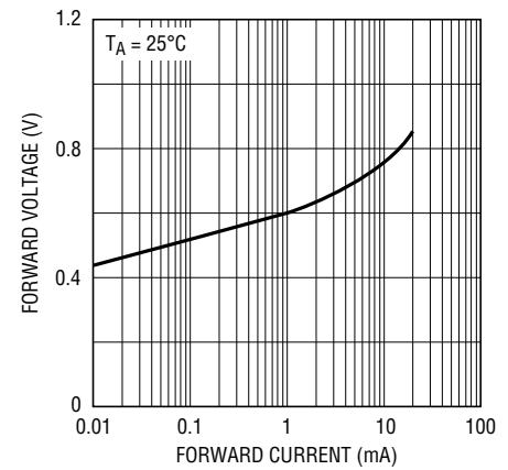
Forward Characteristics
