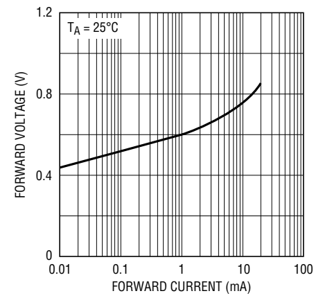
Forward Characteristics
