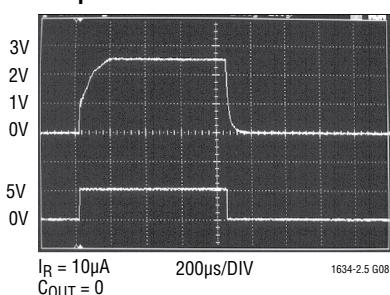
Response Time
