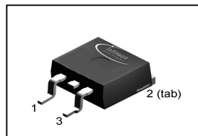
PG-TO263-3-2
