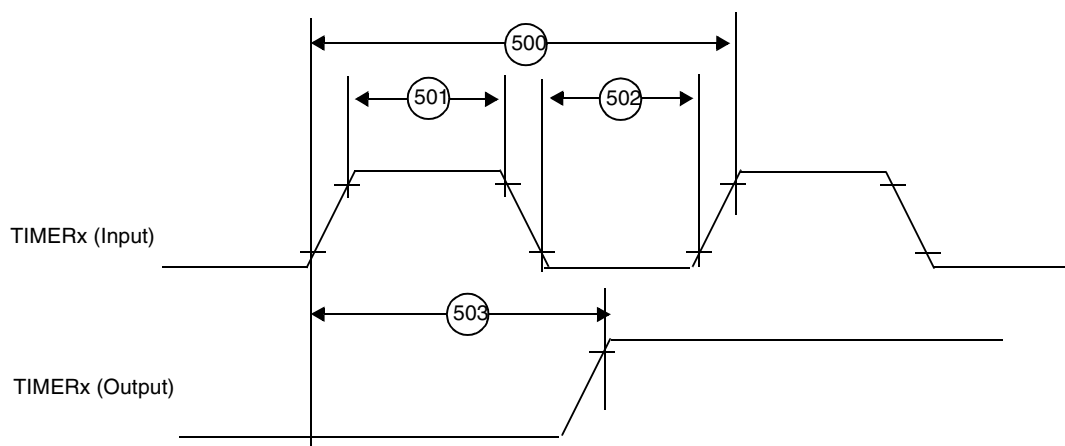
Figure 2-17. Timer Timing
