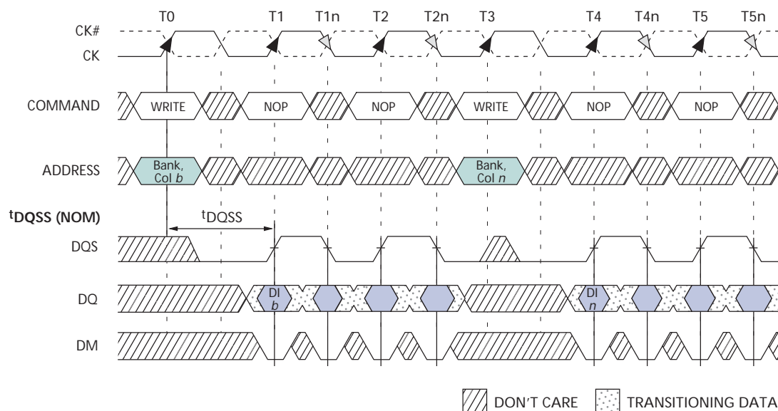
Figure 38: Nonconsecutive WRITE-to-WRITE
