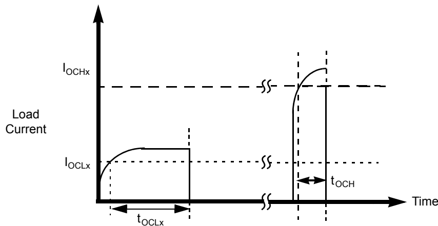
Figure 5. Overcurrent Shutdown
