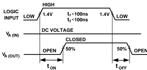
t_{\text{ON}}/t_{\text{OFF}} Timing Diagram
