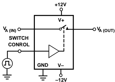
Test Circuit for t_{\text{ON}}/t_{\text{OFF}} Timing Specification, t_{\text{ON}}/t_{\text{OFF}} Switching Response, and ON/OFF Transition Photos
