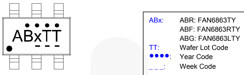
Figure 3. Top Mark
