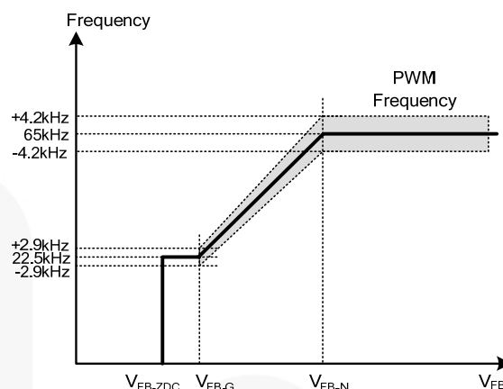
Figure 25. PWM Frequency
