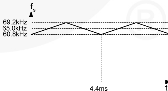
Figure 27. Frequency Hopping
