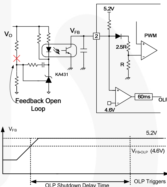
Figure 29. OLP Operation
