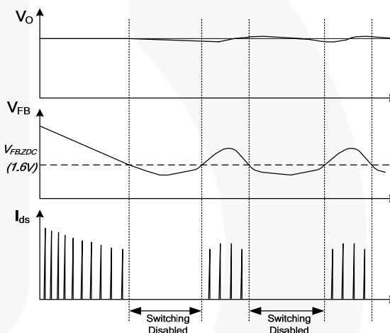
Figure 26. Burst-Mode Operation
