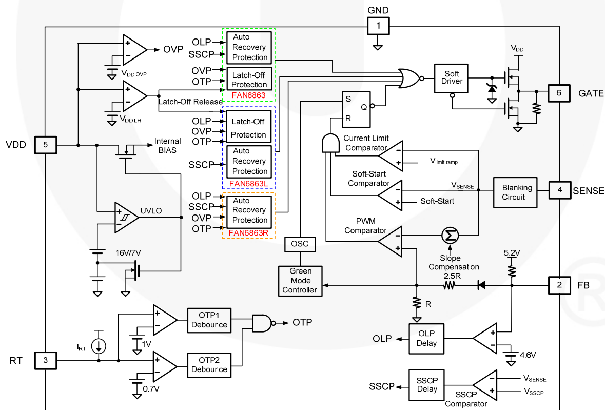
Figure 2. Block Diagram
