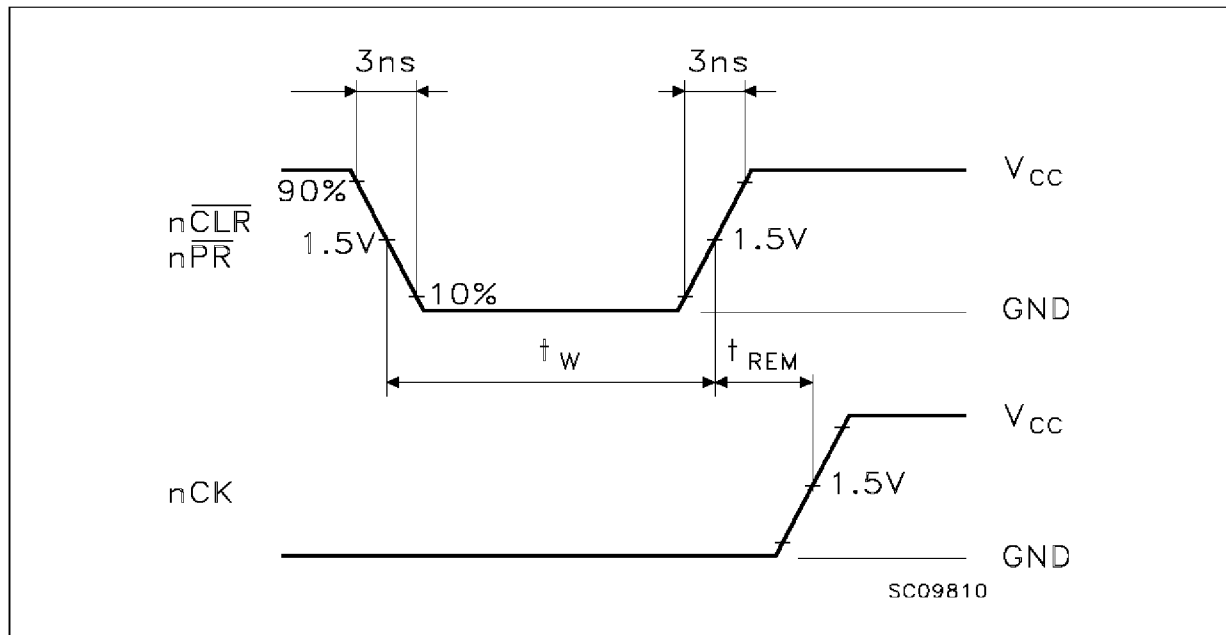
WAVEFORM 3: RECOVERY TIMES ( f=1\text{MHz} ; 50% duty cycle)
