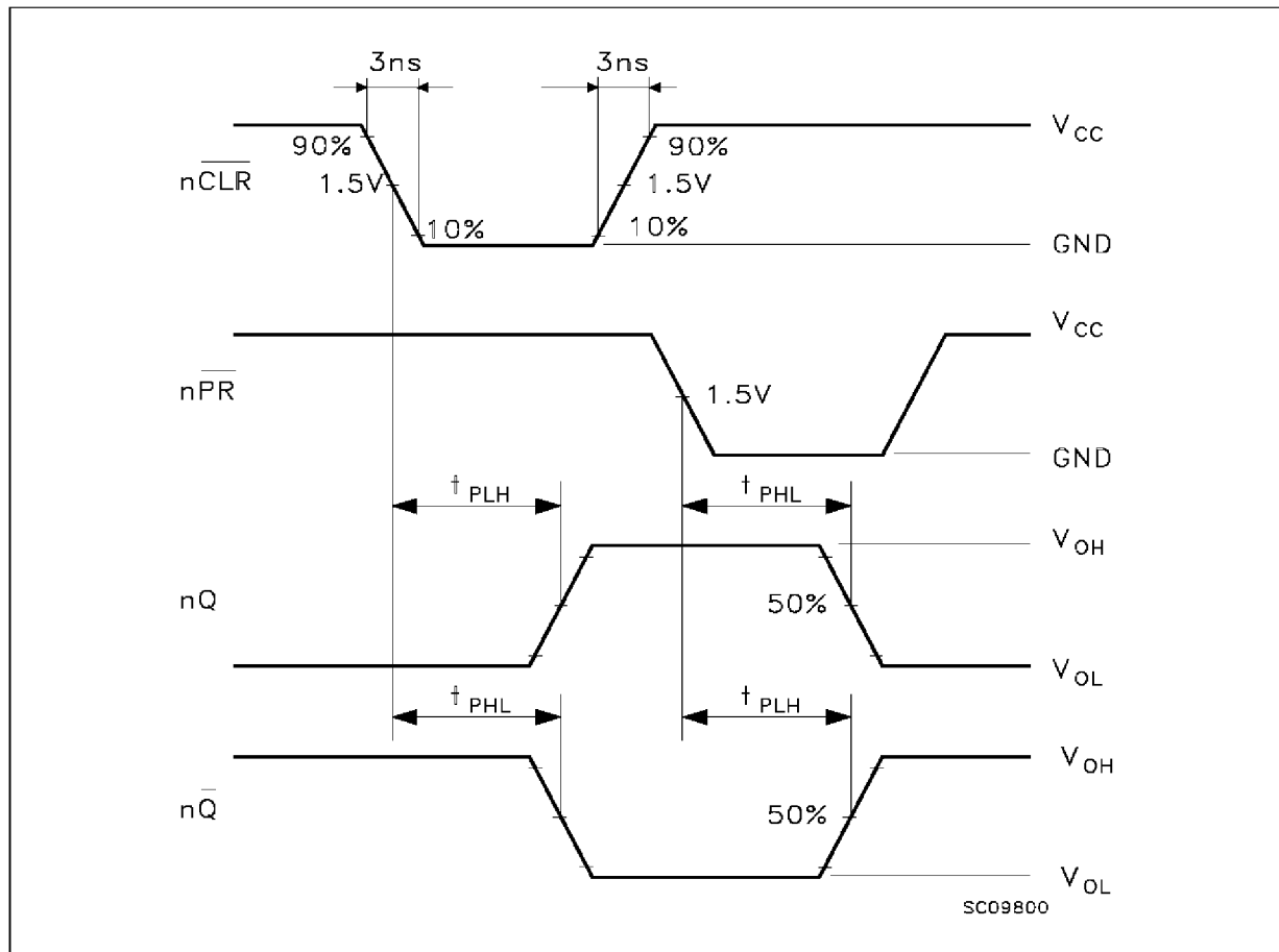
WAVEFORM 2: PROPAGATION DELAYS ( f=1\text{MHz} ; 50% duty cycle)
