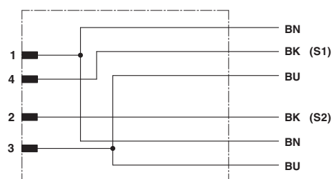
Contact assignment of the M8 Y distributor
