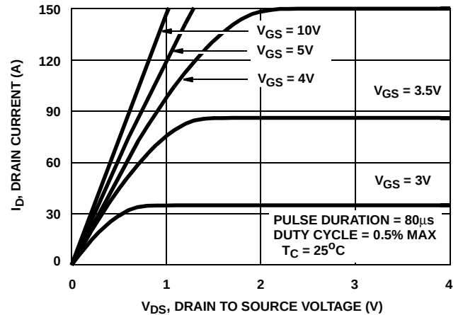
FIGURE 8. SATURATION CHARACTERISTICS
