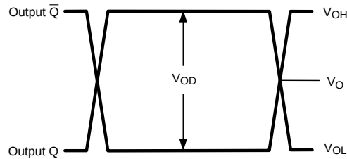
Figure 34. Output Swing
