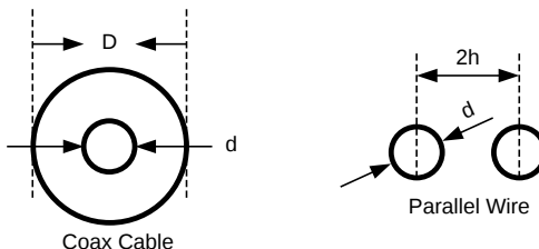
Figure 37. Cable Types
