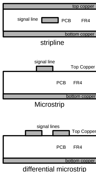
Figure 38. PCB Lines
