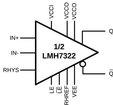
Figure 2. Schematic
