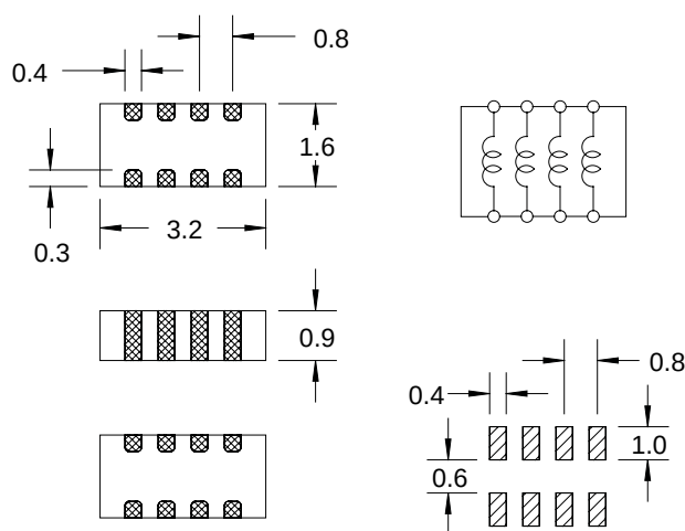
Pad Layout
