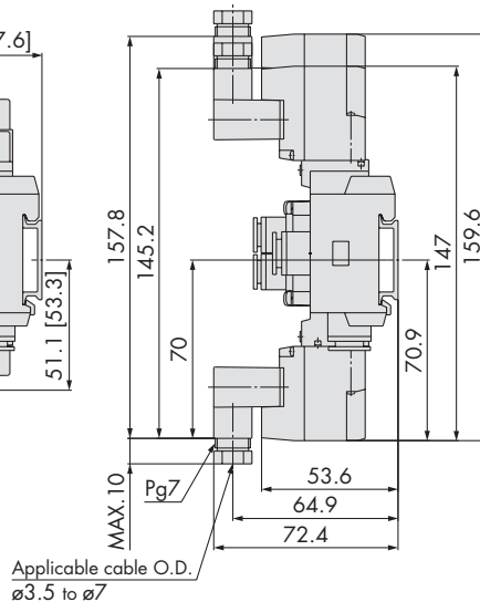
M plug connector (M)
