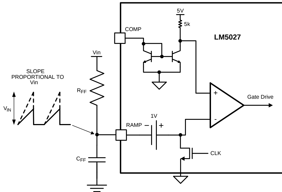
Figure 26. Feed-Forward Voltage Mode Configuration
