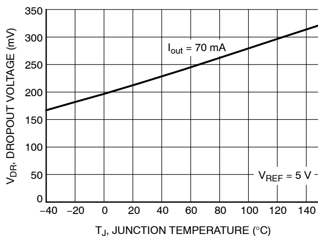
Figure 10. Dropout Voltage V_{DR} vs. Junction Temperature T_J
