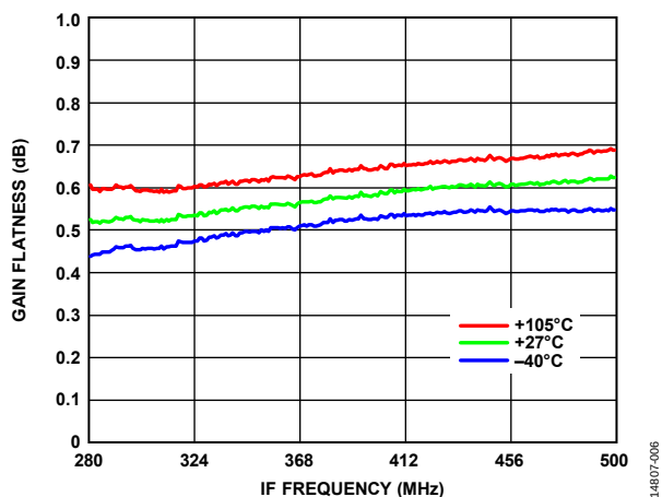
Figure 6. Gain Flatness vs. IF Frequency, Fixed LO Frequency of 2000 MHz, 280 MHz IF Frequency Window
