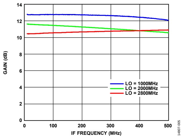
Figure 5. Gain vs. IF Frequency, RF Sweep with Fixed LO, RF to IF Roll-Off
