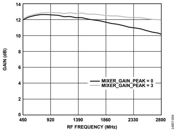
Figure 4. Gain vs. RF Frequency for Various MIXER_GAIN_PEAK (Register 0x003A, Bits[1:0]) Settings
