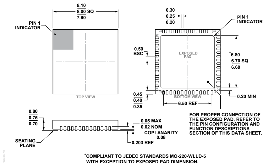
Figure 66. 56-Lead Lead Frame Chip Scale Package [LFCSP] 8 mm × 8 mm Body and 0.75 mm Package Height (CP-56-16)
