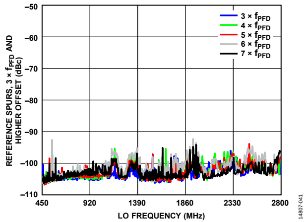
Figure 41. Reference Spurs, 3 \times f_{PFD} and Higher Offset vs. LO Frequency
