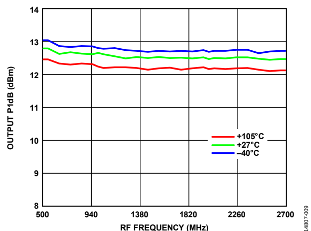
Figure 9. Output P1dB vs. RF Frequency
