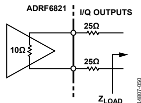
Figure 51. IF Output Schematic
