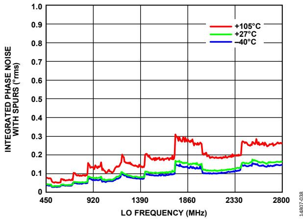
Figure 38. 100 Hz to 10 MHz Integrated Phase Noise with Spurs vs. LO Frequency
