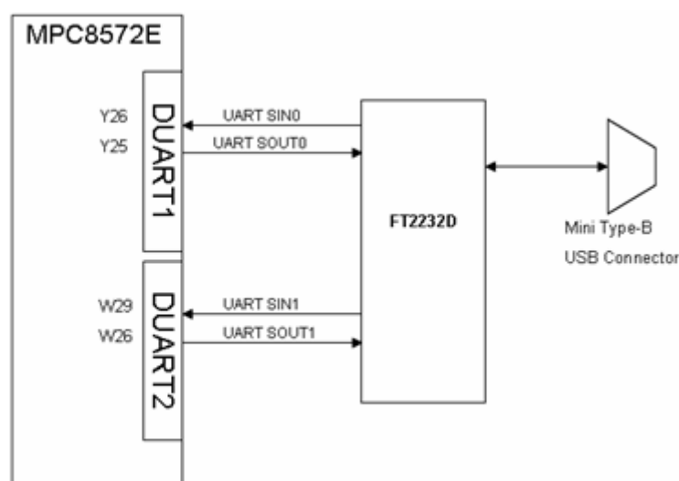
Figure 5-6. DUART Connectivity
