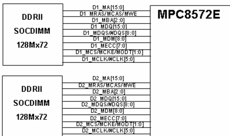
Figure 5-1. DDR2 Connectivity
