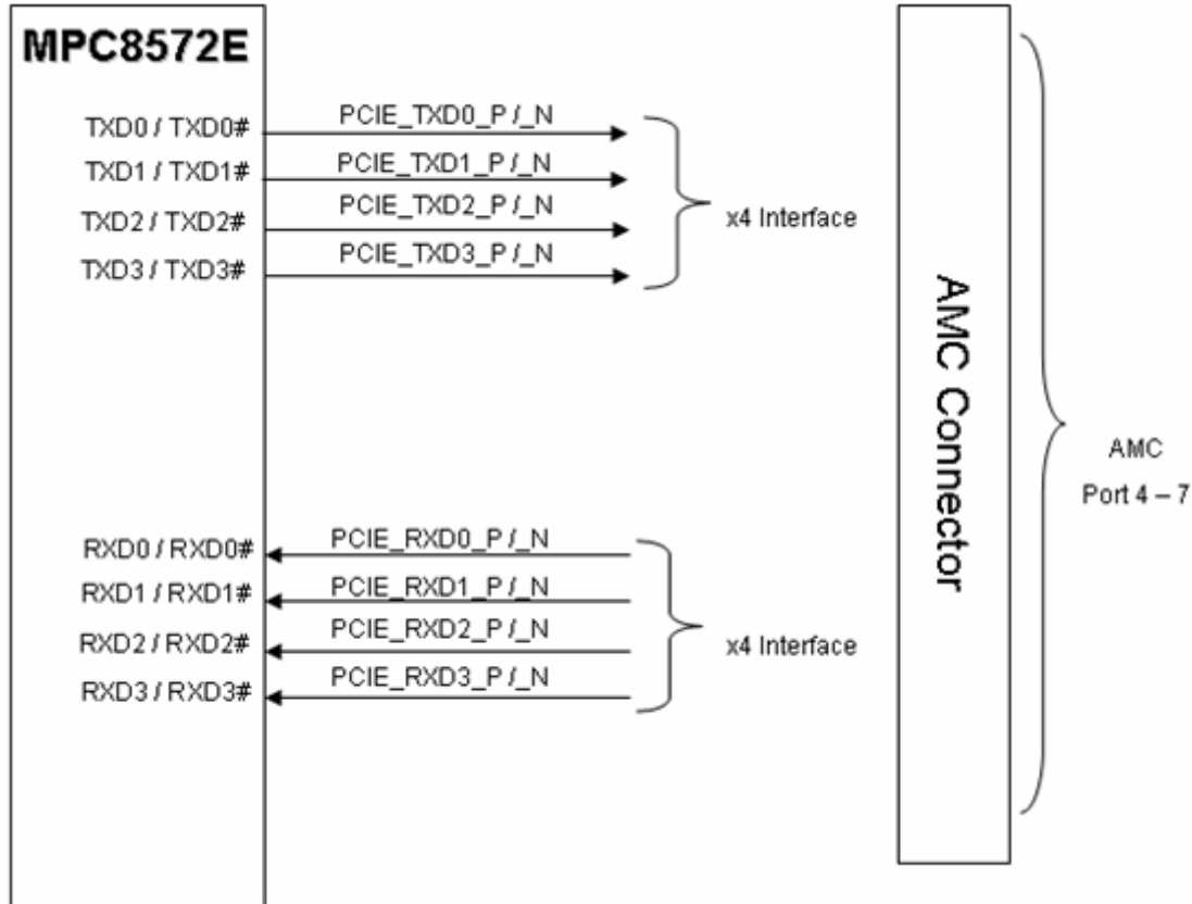
Figure 5-4. PCI-Express Connectivity
