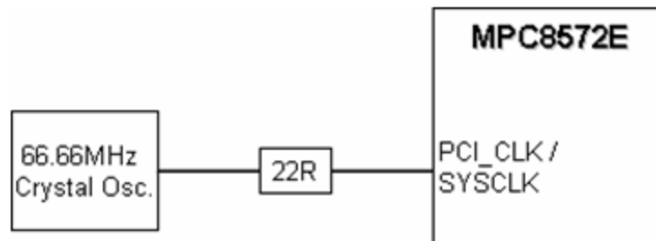
Figure 5-10. SYSCLK Configuration
