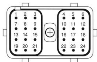
In-line Receptacle
