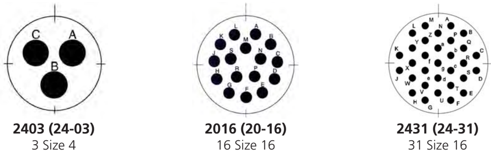
Cavity identification shown from rear socket side
