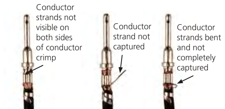
Unacceptable Crimps
