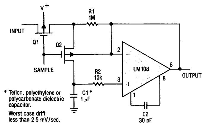
Sample and Hold
