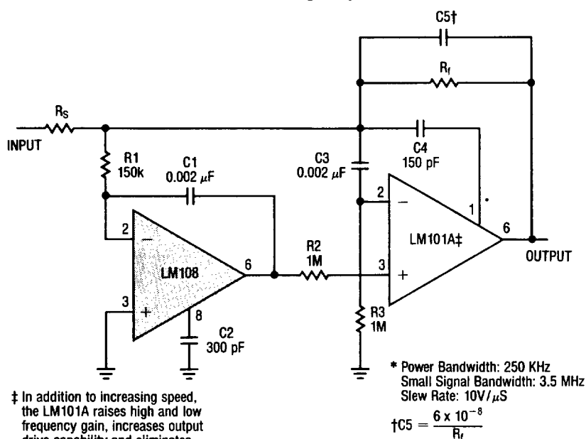
Fast* Summing Amplifier
