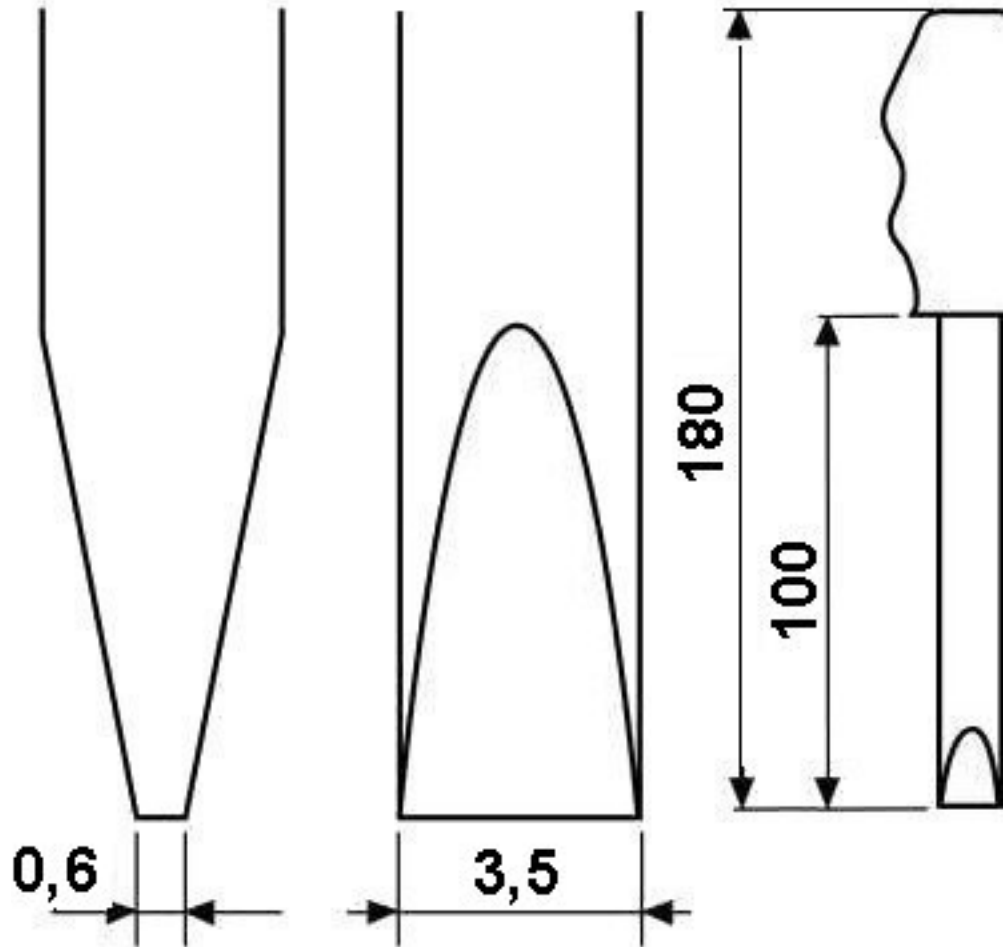
Dimensioned drawing
