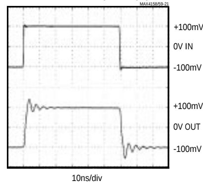
MAX4158/MAX4159 SMALL-SIGNAL PULSE RESPONSE (C L = 20pF)
