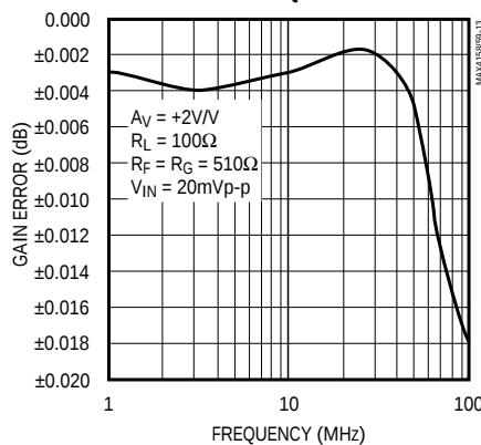
MAX4258/MAX4259 CHANNEL-TO-CHANNEL GAIN MATCHING vs. FREQUENCY
