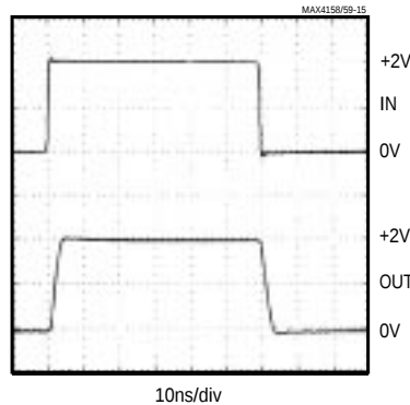
MAX4158/MAX4159 LARGE-SIGNAL PULSE RESPONSE
