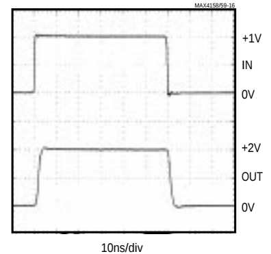
MAX4258/MAX4259 LARGE-SIGNAL PULSE RESPONSE
