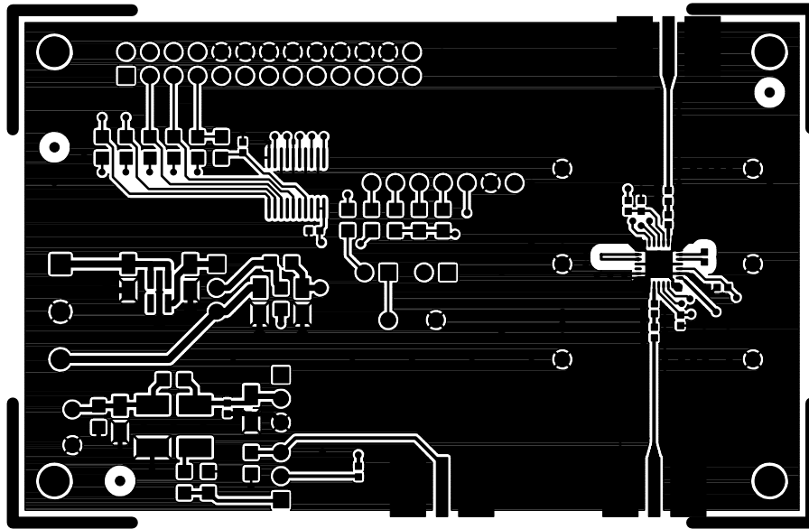
Figure 39. Si4133WM Component
