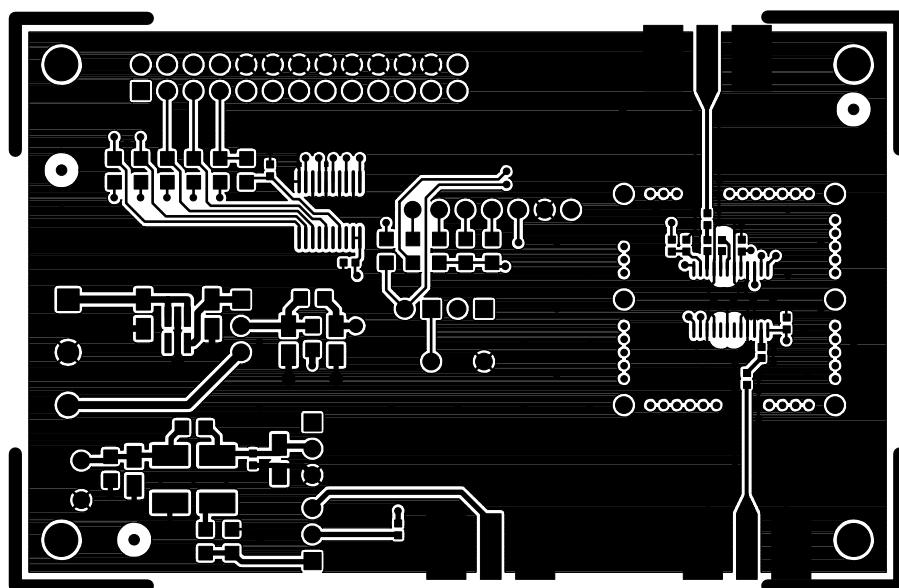
Figure 49. Si4136BT Component
