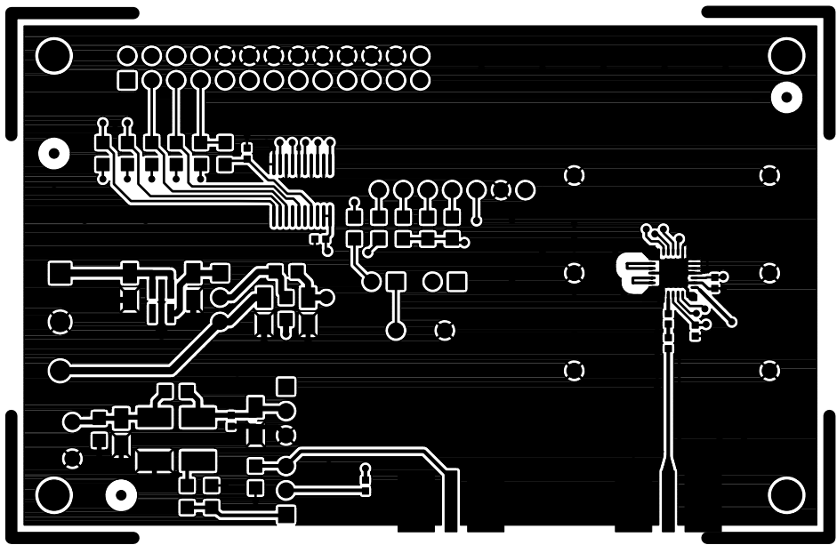
Figure 34. Si4113GX5-BM Component
