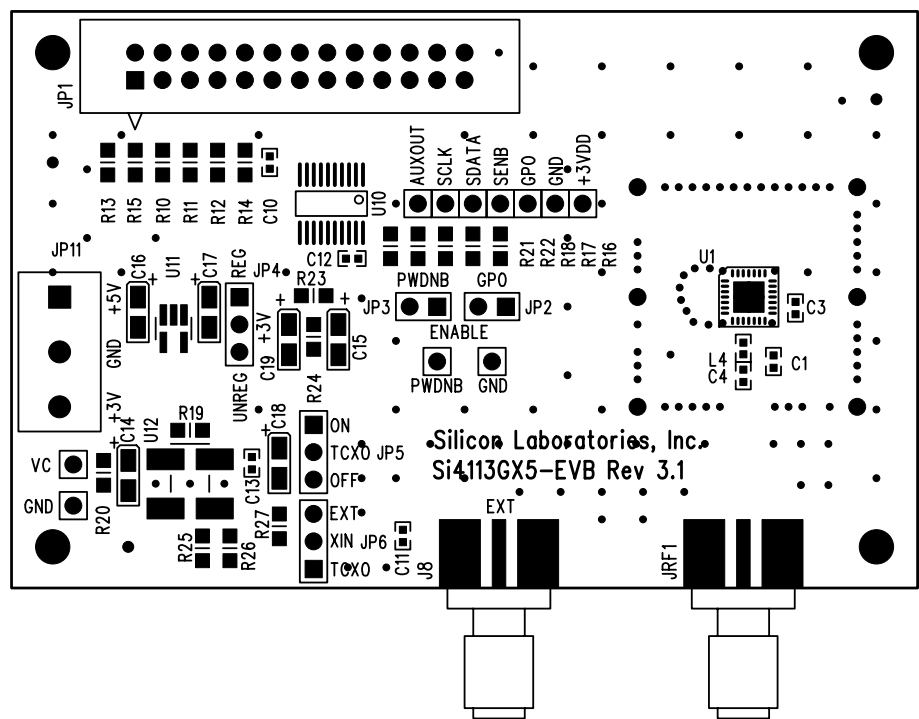
Figure 33. Si4113GX5-BM Silkscreen
