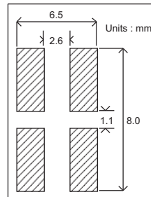
Figure 17. Si4133W MLP (1 of 2)
