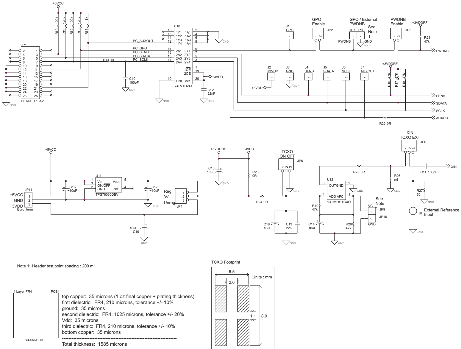
Figure 15. Si4113GX5 MLP (1 of 2)
