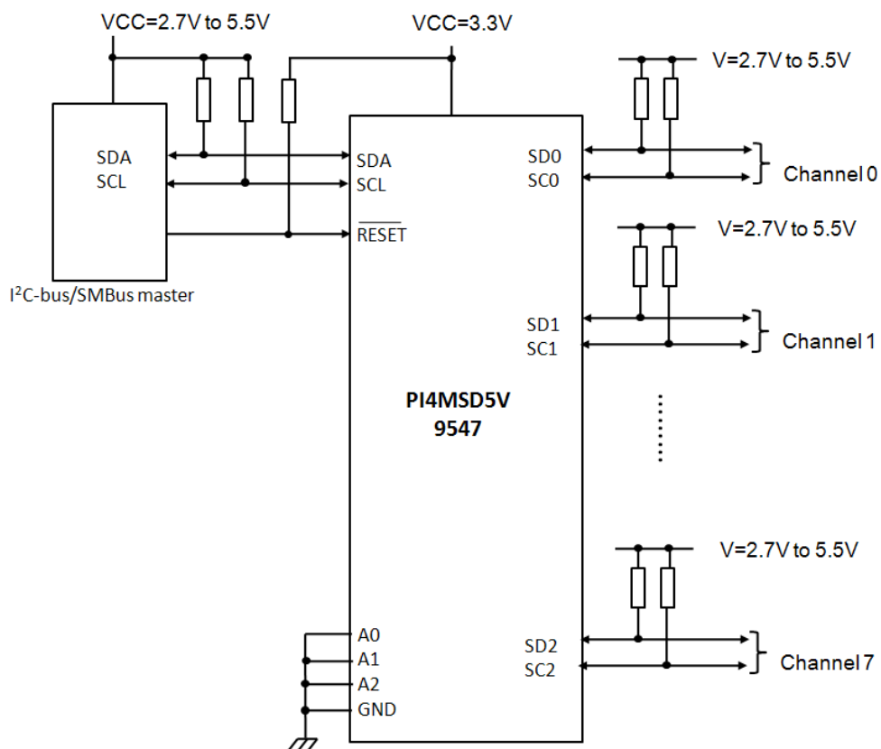
Figure 3. Typical Application
