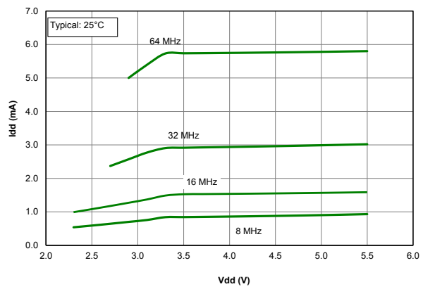
Figure 39-45. I_{DD} , ECH Oscillator, Typical, PIC18F24/25K40 only
