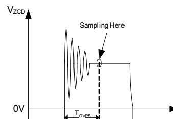
Figure 9: ZCD Voltage and OVP Sampling
