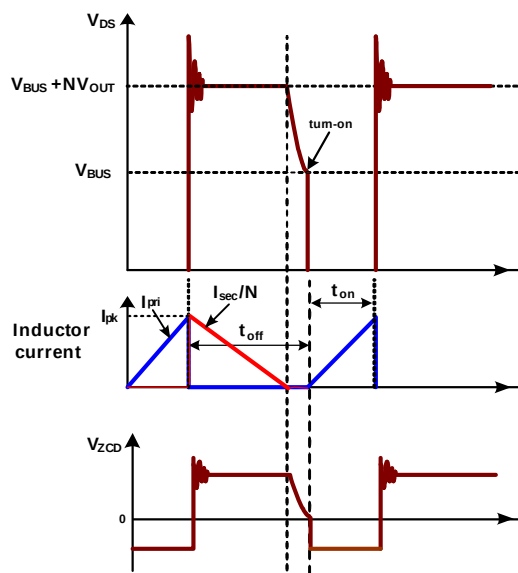
Figure 2: Boundary-Conduction Mode
