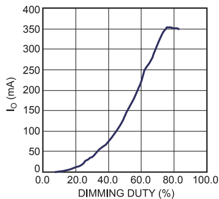
Triac Dimming Curve
