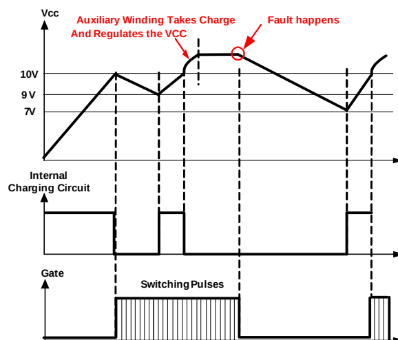
Figure 5: VCC Timing Sequence
