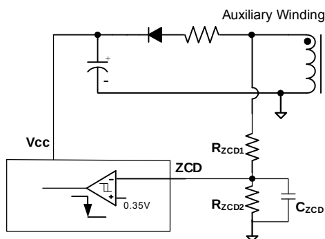
Figure 3: Zero-Current Detector
