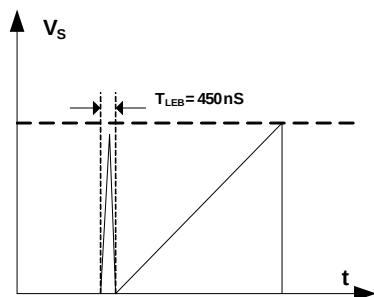
Figure 7: Leading-Edge Blanking
