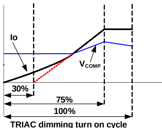
Figure 12: Dimming Curve
