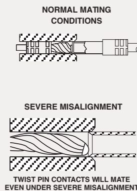
Figure 2 - Illustrates the Twist Pin features, as well as mating & severe misalignment conditions.
