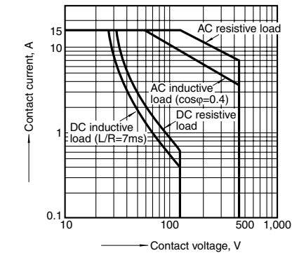
Switching capacity range (1 Form C)
