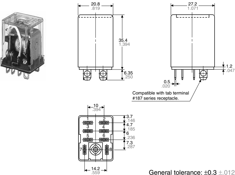
External dimensions
