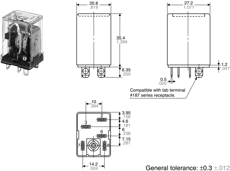
External dimensions
