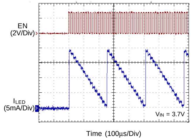
Dimming Operation
