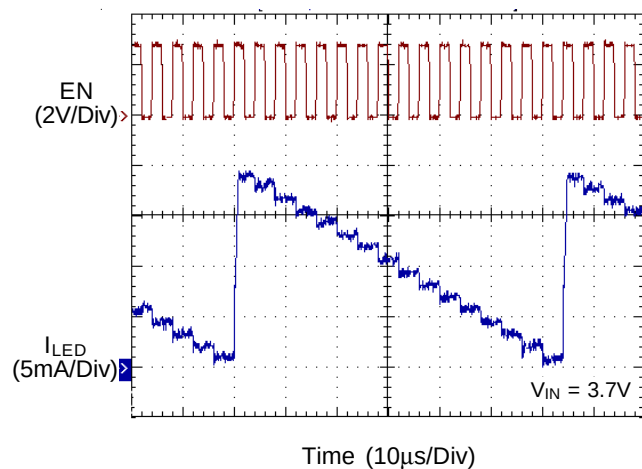
Dimming Operation
