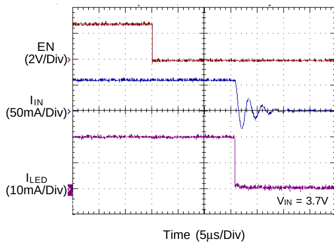
Turn-Off
