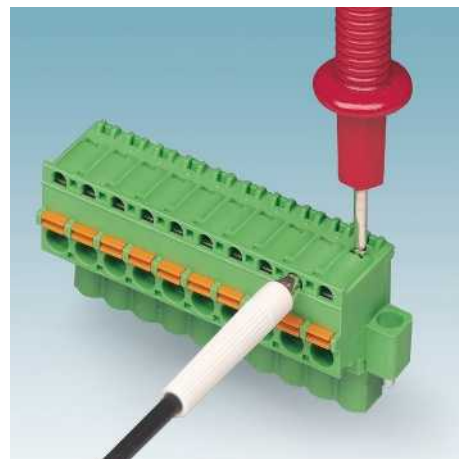
Integrated test connections
