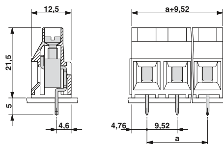
Drilling diagram
