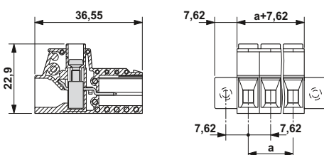
Type: IPC 5/...-ST-7,62 with IPC 5/...-G-7,62 Conductor cross section: 10 mm²
