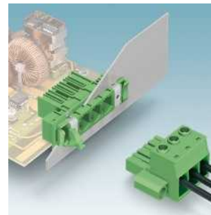
PC 16 series: feed-through headers, solder and screw connection, up to 76 A, 10.16 mm pitch DFK-PC 16... Page 574
