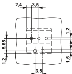
Drilling diagram for MKDSFW 1,5/3-3,5
