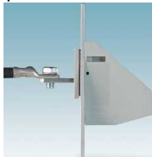
HDFK 50-VP/HDFK 95-VP series: screw connection, up to 232 A, molded terminal blocks HDFK 50...VP...
