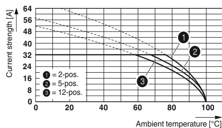
Type: IPC 5/...-ST-7,62 with PC 5/...-ST1-7,62 Conductor cross section: 6 mm²
