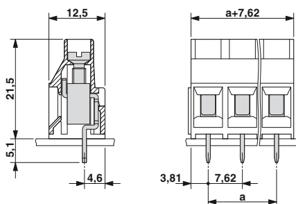
Drilling diagram
