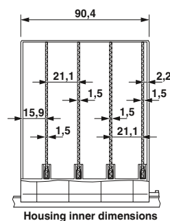
Housing inner dimensions
