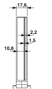
Housing inner dimensions
