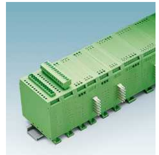
UEGM... component housings Shell housing with variable connection technologies Page 724
