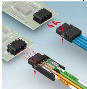
Miniature plugs and headers with 2.5 mm pitch PTSM 0,5... Page 55 PTPM Page 55
