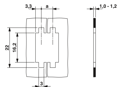
Panel feed-through for CIOC...FL, see page 65. Dimension a = 6.5 mm
