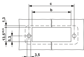
Sheet metal cutout dimensions for IC-DFR..., see page 350.
