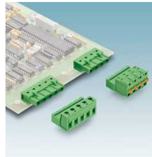
Inverted plug with screw and spring connection, 7.62 mm pitch GIC 2,5/...-ST(GF)-7,62 Page 338 GFKIC 2,5/...-ST-7,62 Page 341
