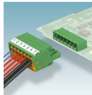
Plugs with IDC displacement connection, 5.0/5.8 mm pitch QC 1,0/...-ST(F)-5,08 Page 290 QC 1,5/...-ST(F)-... Page 292
