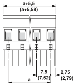
Dimensional drawing
