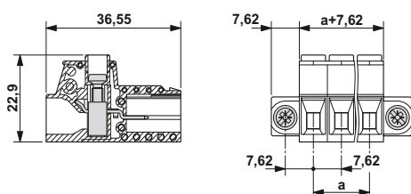
Type: IPC 5/...-ST-7,62 with PC 5/...-ST1-7,62 Conductor cross section: 6 mm²
