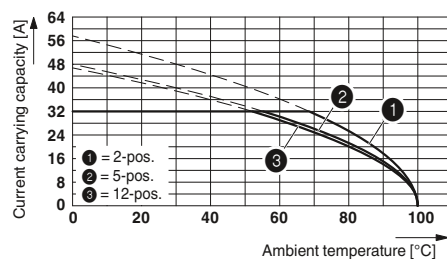
Type: IPC 5/...-ST-7,62 with IPC 5/...-G-7,62 Conductor cross section: 6 mm²
