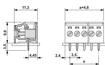
Drilling diagram
