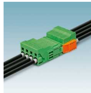
PC 5 series: inverted plugs/headers, spring connection, up to 41 A, 7.62 mm pitch ISPC 5/... Page 544
