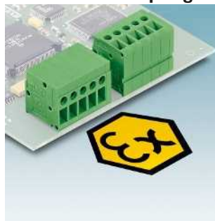
Horizontal and vertical PCB terminal blocks with front connection with 5.0 mm pitch, 2.5 mm² connection cross section FRONT 2,5/...-EX Page 158
