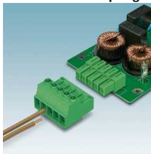
PC 5 series: inverted plugs/headers screw connection, up to 41 A, 7.62 mm pitch IPC 5/... Page 526
