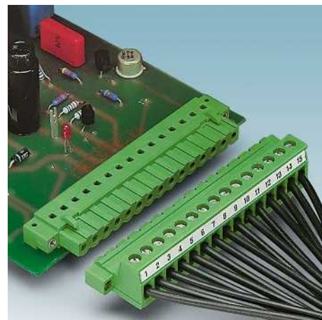
6. IC 2,5/... STF with screw flange for vibration-resistant connection with IC 2,5/... GF inverted headers.
