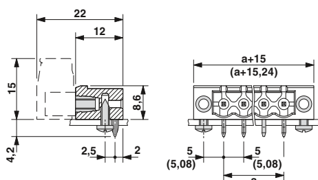
Drilling diagram
