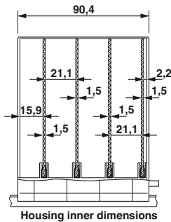
Housing inner dimensions
