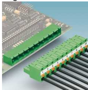
Plugs with push-in spring connection, 7.5/7.62 mm pitch, plug-in direction parallel to the conductor axis GFKC 2,5/...-ST(F)-... Page 340
