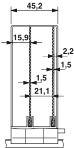
Housing inner dimensions
