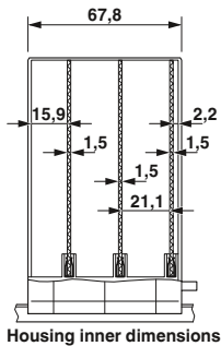
Housing inner dimensions
