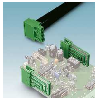
Headers with 5.08 mm pitch orthogonal plug-in direction MSTBO 2,5/...-G-5,08 Page 320
