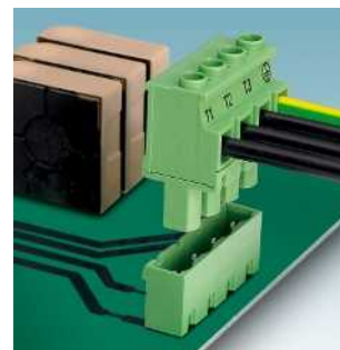
HV series: vertical connection direction, screw connection, up to 16 A, 7.62 mm pitch, 600 V UL GMVSTBR/W 2,5 HV... Page 500
