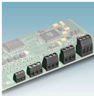
Through hole reflow applications with screw connection 3.5/3.81/5.0/5.08 mm pitch MKDS Page 75
