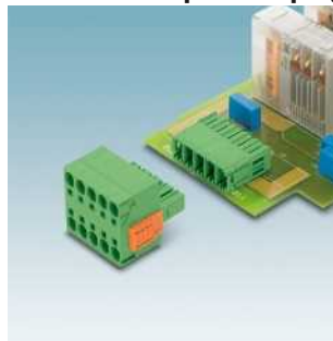
PC 5 series: plugs with double spring connection, up to 41 A, 7.62 mm pitch TSPC 5... Page 532
