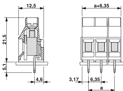
Drilling diagram
