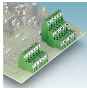
Double and three-level PCB terminal blocks with 3.5/3.81 mm pitch MKKDS 1/... Page 85 MK3DS 1/... Page 87
