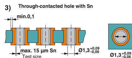
Structure of the metal-plated hole for EMSTB(A) 2,5/...-G(F)-... and EMSTBV(A) 2,5/...-G(F)-...
