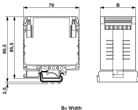
6-pos. with screw connection, width: 22.5 mm, 25 mm, and 27.5 mm
