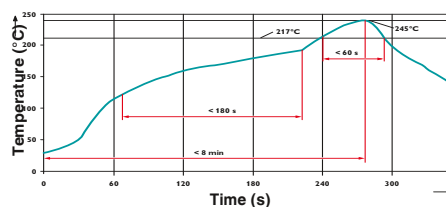
Lead-free reflow soldering profile (SnAgCu)
