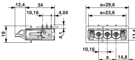
Drilling diagram
