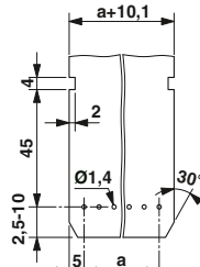
PCB cutout for ICV 2,5/...-G-5,08 with FLRP-ICV 80, see page 333.
