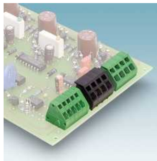
Angled PCB terminal blocks with spring-cage connection ZFKDS 1-3,81 Page 129 ZFKDS 2,5-5,08 Page 135
