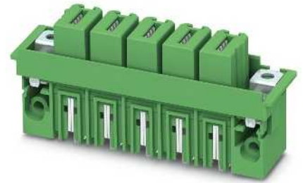
Vertical, for fixing in the housing panel with shield connection, 600 V UL approval
