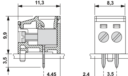
MKDSFW 1,5/2-3,5 with locating pin, see page 87.
