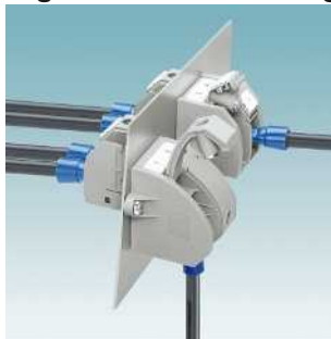
RW 5 series: bolt connection, up to 76 A, connection: vertical and horizontal RW 5...
