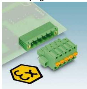
Plugs with push-in spring connection for the Ex area, 5.08/7.62 mm pitch FKC 2,5/...STF5,08 EX Page 371 GFKC 2,5/ 2-STF-7,62 EX Page 381
