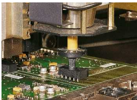
Component placed on the PCB
