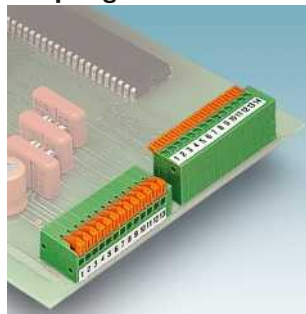
Horizontal and vertical push-in spring connection, 2.54/3.81/5.08/7.62 mm pitch FFKDS(A)... Page 145
