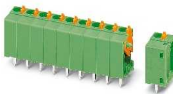
5.08 mm pitch, with shortened opening lever, conductor connection vertical to the PCB
