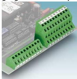
Compact design, 5.0 mm pitch, 1.5 mm² connection cross section ZFKDS 1,5C-5,0 Page 131
