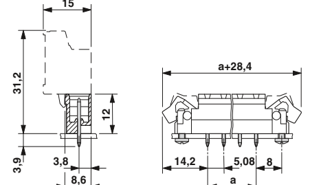
Drilling diagram
