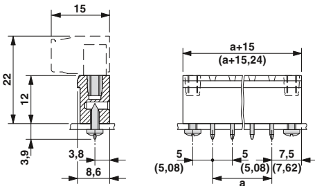
Drilling diagram
