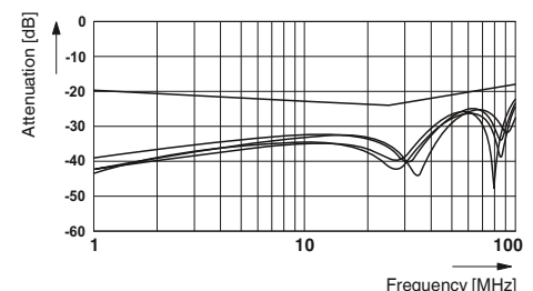
Reflection loss for PTPM plug with Ethernet cable
