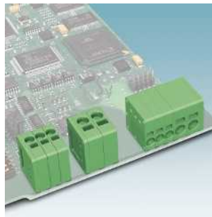
Horizontal and vertical push-in spring connection, 3.5/5.0 mm pitch SPT 1,5/...-3,5 Page 141 SPT 2,5/...-5,0 Page 143
