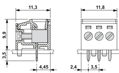
MKDSFW 1,5/3-3,5 with locating pin, see page 87.
