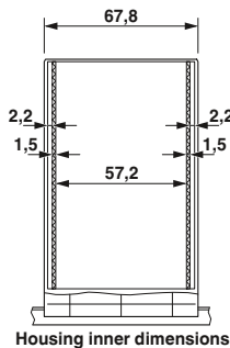
Housing inner dimensions
