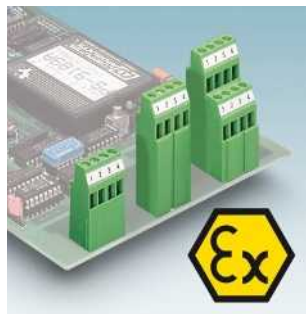
High PCB terminal blocks with 5.0/5.08 mm pitch MKKDSH 3/...-EX Page 157 MK3DSH 3/...-5,08-EX Page 157 MK3DSMH 3/...-5,08-EX Page 157
