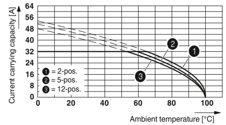
Type: ISPC 5/...-STGCL-7,62 with SPC 5/...-ST-7,62
