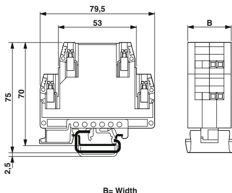
8-pos. with screw connection, width: 20 mm
