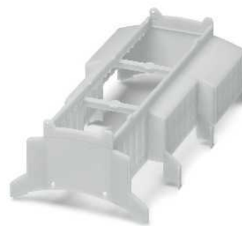
Modular upper part for customer-specific configuration 161.6 mm wide = 9 pitches
