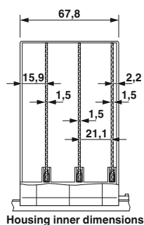
Housing inner dimensions
