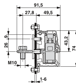
Drilling diagram
