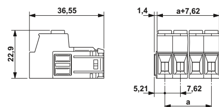
Type: IPC 5/...-ST-7,62 with IPC 5/...-G-7,62 Conductor cross section: 6 mm²
