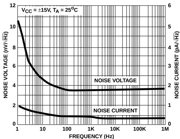
FIGURE 6. NOISE CHARACTERISTICS
