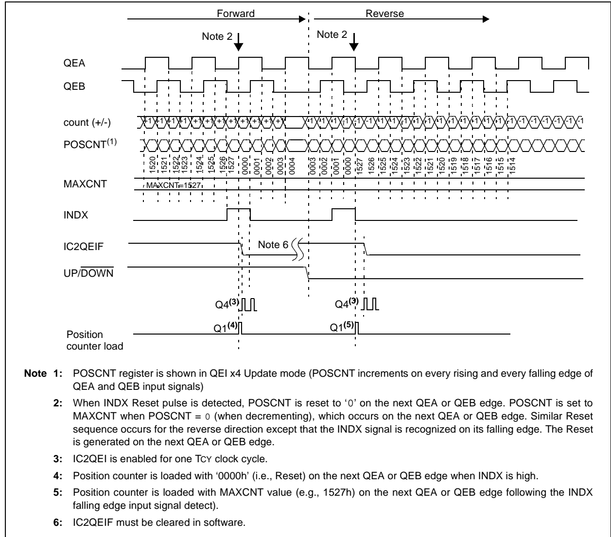
FIGURE 16-11: QEI MODULE RESET TIMING WITH THE INDEX INPUT
