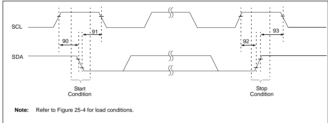
FIGURE 25-17: SSP I 2 C BUS START/STOP BITS TIMING WAVEFORMS
