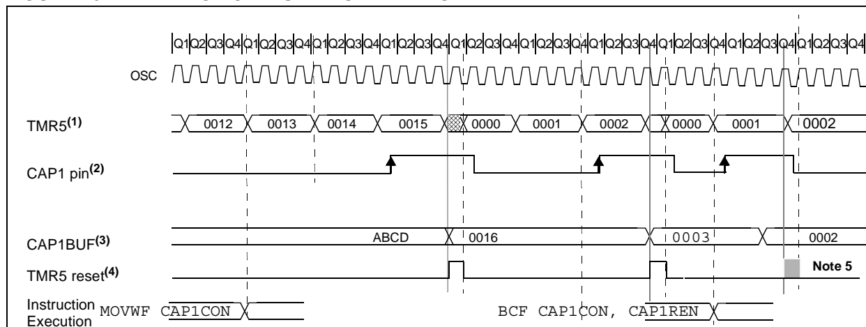
FIGURE 16-4: EDGE CAPTURE MODE TIMING
