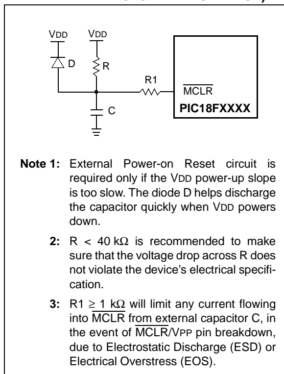
FIGURE 4-2: EXTERNAL POWER-ON RESET CIRCUIT (FOR SLOW VDD POWER-UP)
