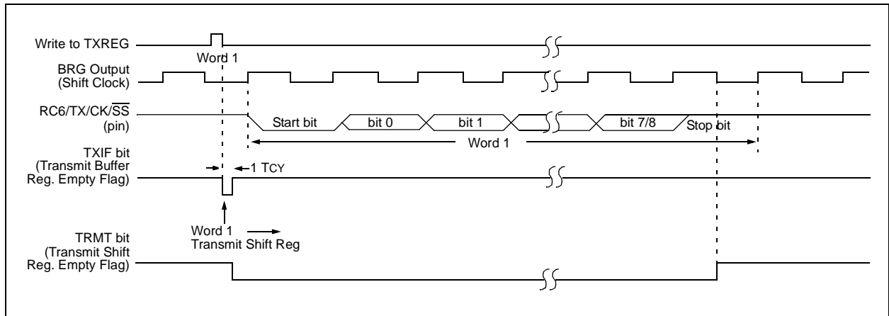
FIGURE 19-3: ASYNCHRONOUS TRANSMISSION
