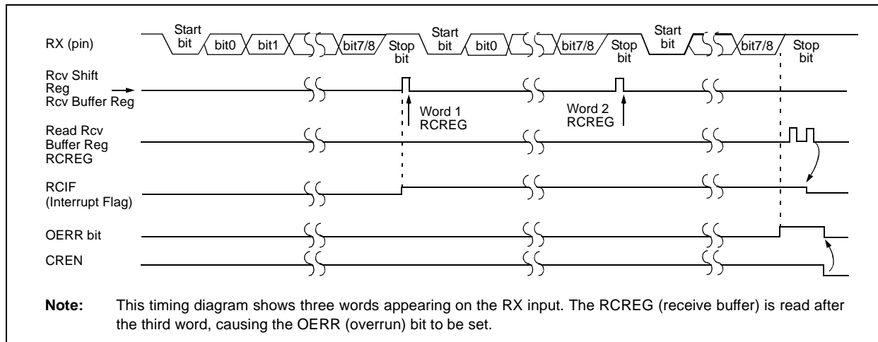
FIGURE 19-6: ASYNCHRONOUS RECEPTION
