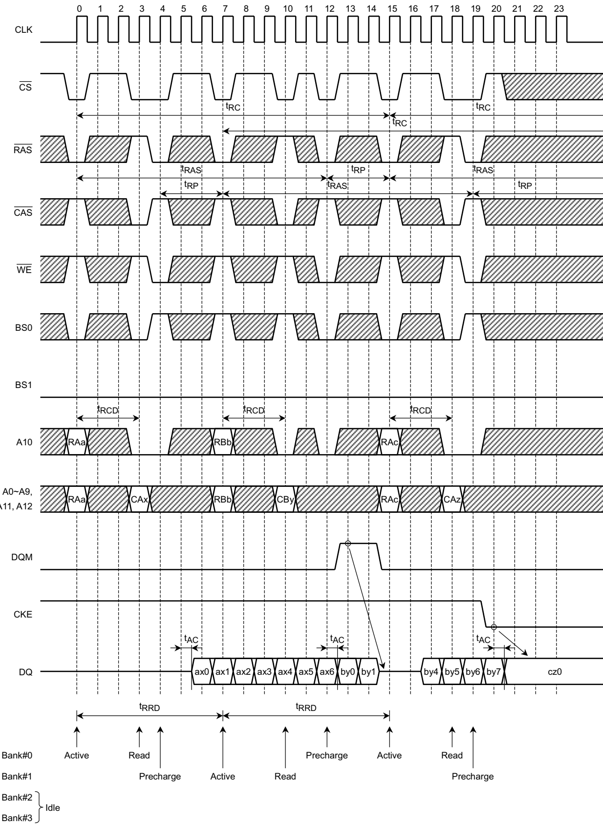
Figure 3. Interleaved Bank Read (Burst Length = 8, \overline{\text{CAS}} Latency = 3)
