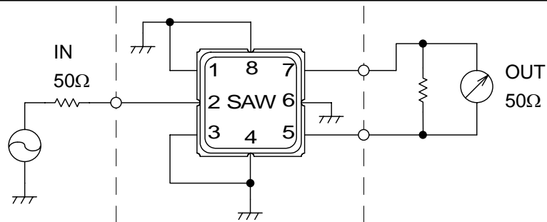
Fig.1 Measuring circuit
