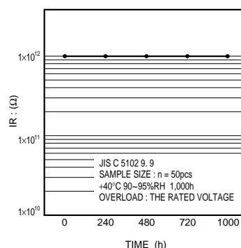
Fig.27 Insulation resistance
