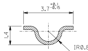
SECT. C-C (SCALE 10 : 1)
