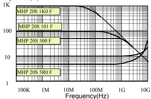
Frequency Characteristics
