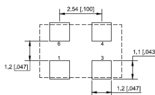
Recommended Land Pattern for CMOS
