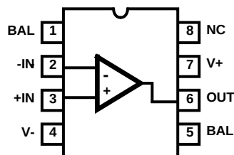
HA-5170 (CERDIP) TOP VIEW
