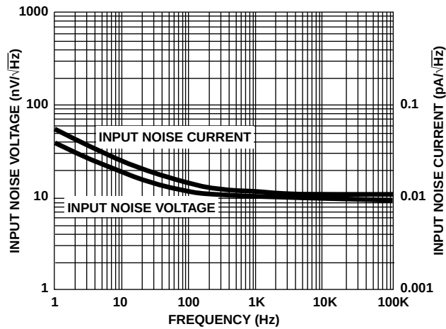
FIGURE 4. INPUT NOISE vs FREQUENCY
