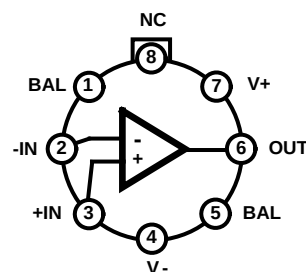
HA-5170 (METAL CAN) TOP VIEW
