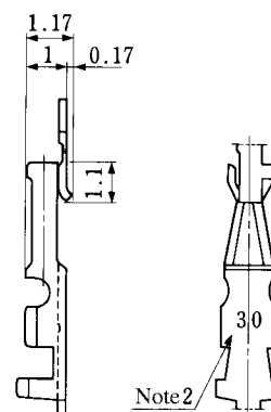
SCFC contact
