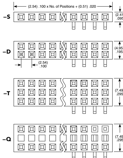
Through-hole
