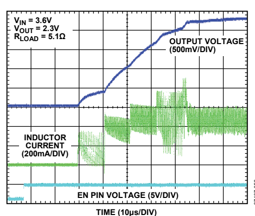
Figure 45. Start-Up Waveform, Heavy Load
